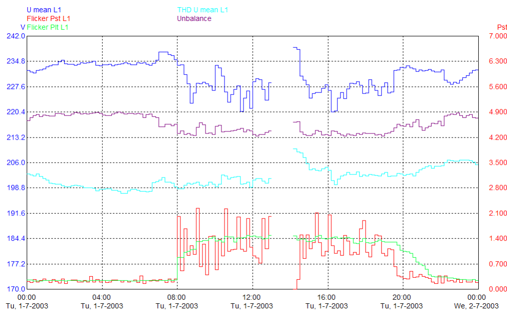
Fig. 3. Several power quality parameters measured at the sawmill over 1 day
