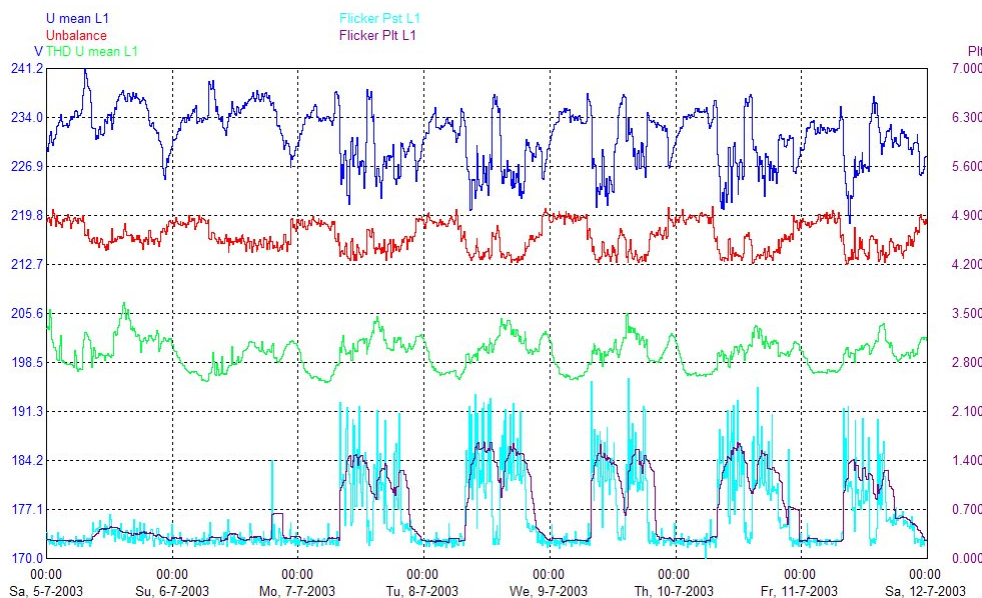
Fig. 4. Several power quality parameters measured at the sawmill over 1 week
