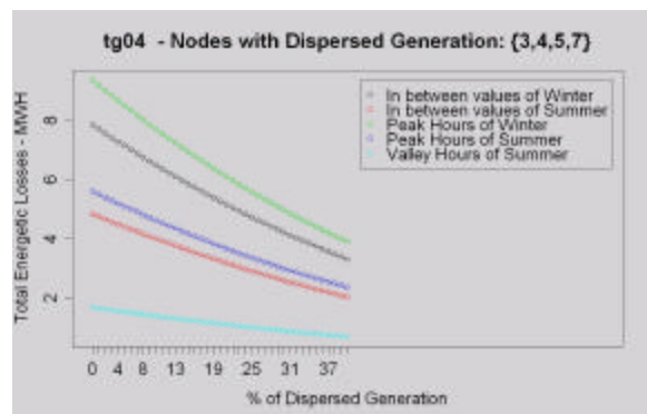
Fig. 17. HV Network – Energetic Losses
