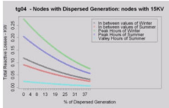
Fig. 14. RMV Network – Reactive Losses
