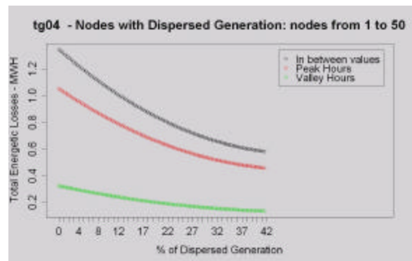
Fig. 20 – UMV Network. Energetic Losses
