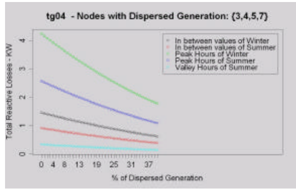
Fig. 13. HV Network – Reactive Losses
