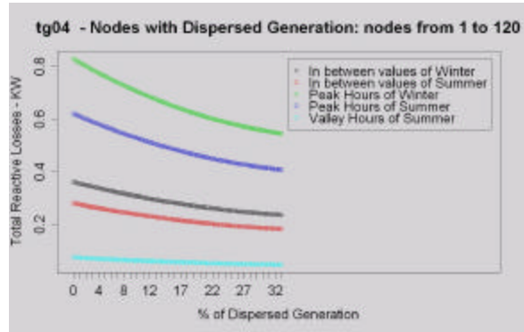
Fig. 15. SUMV Network – Reactive Losses
