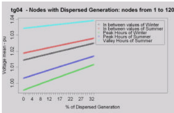
Fig. 7. SUMV Network – Voltage mean
