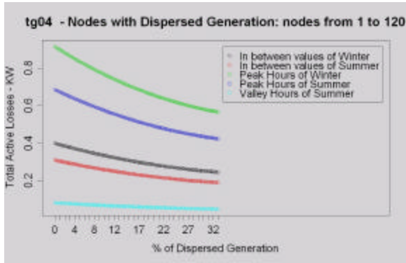
Fig. 11. SUMV Network – Active Losses
