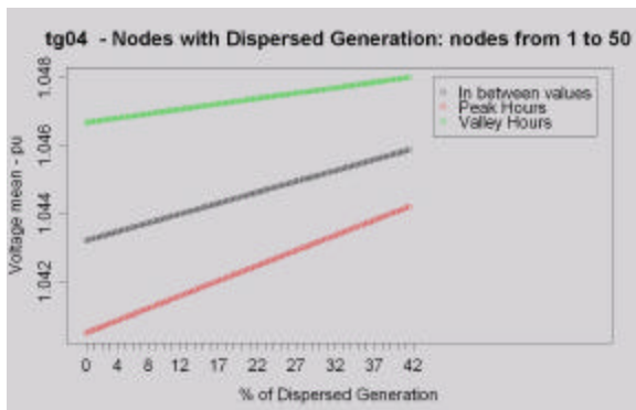
Fig. 8. UMV Network – Voltage mean
