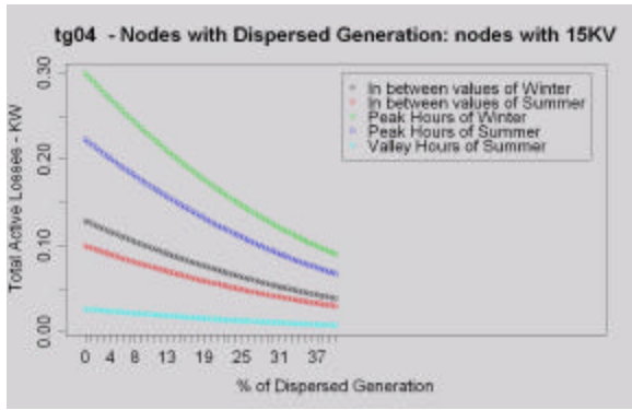
Fig. 10. RMV Network – Active Losses
