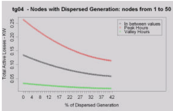
Fig. 12. UMV Network – Active Losses
