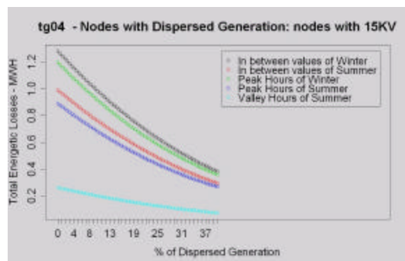
Fig. 18. RMV Network – Energetic Losses
