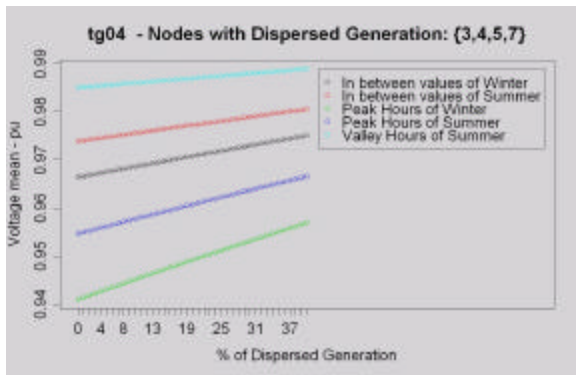
Fig. 5. HV Network – Voltage mean
