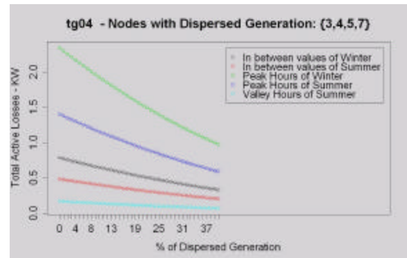
Fig. 9. HV Network – Active Losses
