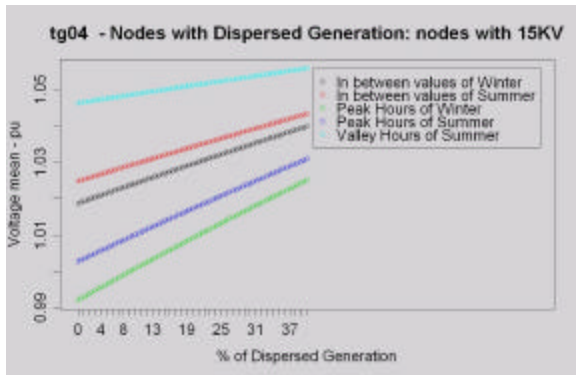
Fig. 6. RMV Network – Voltage mean
