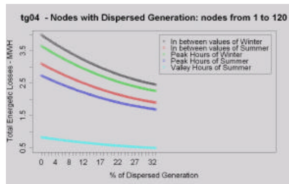
Fig. 19. SUMV Network. Energetic Losses
