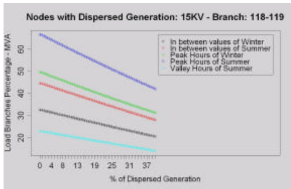
Fig. 22. RMV Network – Load Branches
