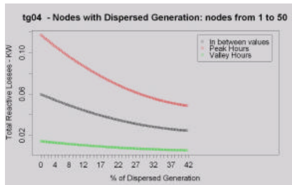
Fig. 16. UMV Network – Reactive Losses
