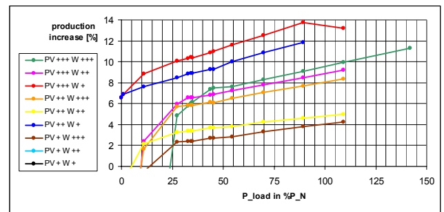
Fig. 4. Production increase versus load power level in several operating conditions for solar radiance and wind speed: +++=maximum, ++=average, +=minimum
