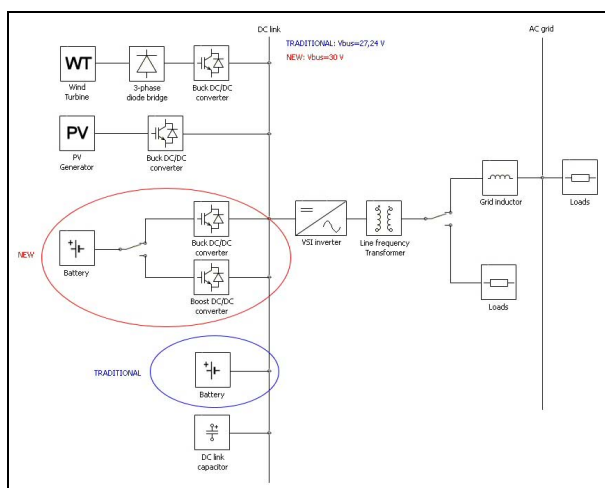
Fig. 3. Traditional and new circuit topologies
